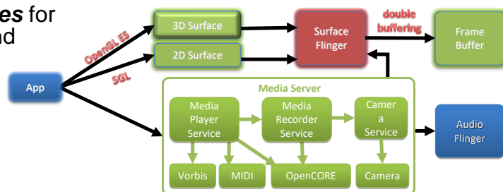
Surface Manager + Media Framework
