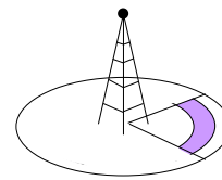
CGI + TA
