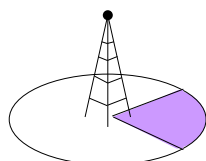
CGI
